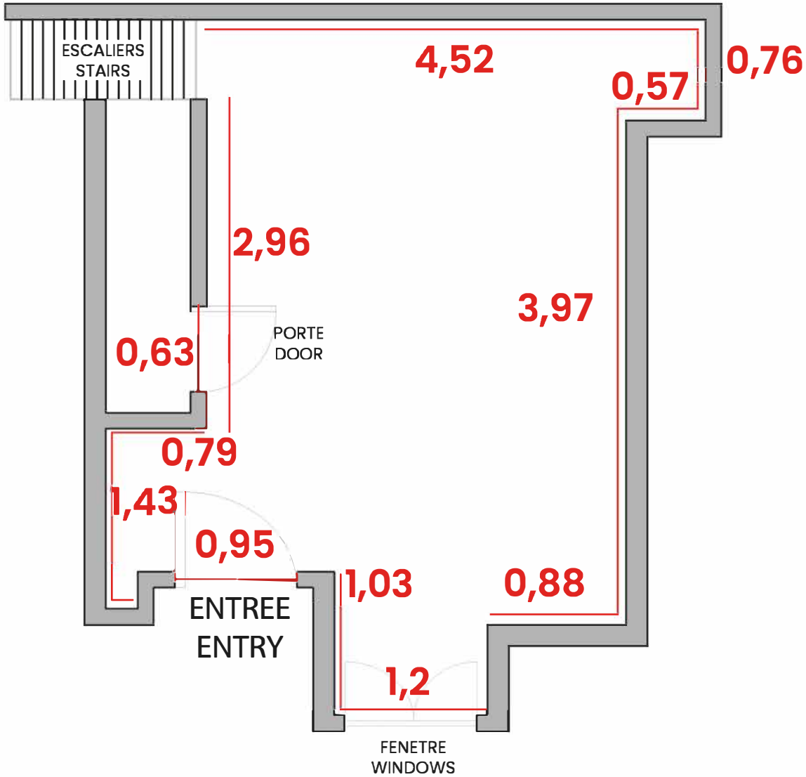
REZ DE CHAUSSEE GROUND FLOOR
