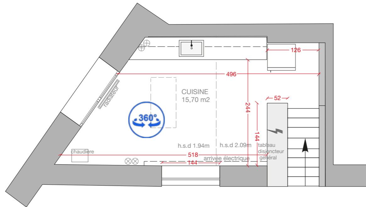
PLAN MEZZANINE
